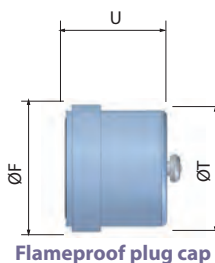
HAWKE Ex SERIES DIMENSIONS (MM)
