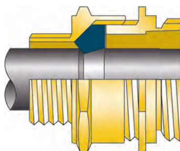
Cable damage as found with cable gland designs incorporating compression / displacements seals
